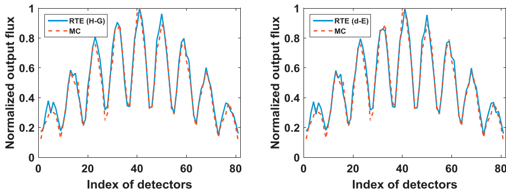
Fig. 2. Comparison between RTE and Monte Carlo (MC). (a) Comparison of normalized fluence obtained from RTE with Henyey–Greenstein phase function and MC simulation; (b) Comparison of normalized fluence obtained from RTE with delta-Eddington function and MC simulation.
